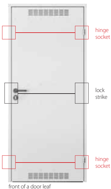
front of a door leaf
