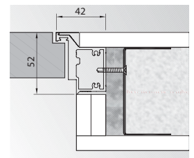
reversed rebate (inward opening)
